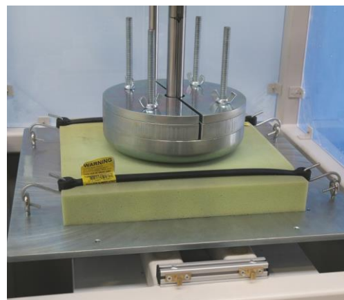
Indentor with weights, Test Sample and Plane Platen
